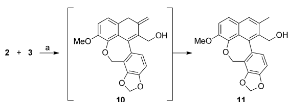
Scheme 3. Domino Sonogashira/carbopalladation/Heck reaction: a) [\text{Pd}(\text{PPh}_3)_4] , tetrabutylammonium fluoride (TBAF)·3 H 2 O, 1,2-dimethoxyethane (DME), 80 °C, 24 h, 50%.
