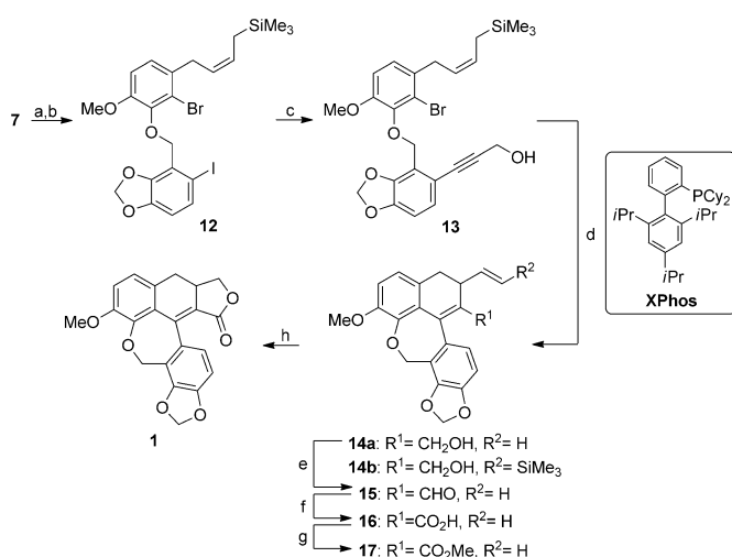
Scheme 4. Synthesis of linoxepin ( 1 ): a) \text{Ph}_3\text{PCH}_2\text{Br} , KO t Bu, \text{ICH}_2\text{SiMe}_3 , THF, 0 °C, 3 days, 68%; b) 5 , K 2 CO 3 , MeCN, 80 °C, 5 h, 99%; c) 3 , [\text{Pd}(\text{PPh}_3)_4] (7 mol%), CuI (10 mol%), Bu 4 NOAc, dioxane, 60 °C, 30 min, 98%; d) Pd(OAc) 2 (5 mol%), XPhos (7.5 mol%), Bu 4 NOAc, DME, 80 °C, 1 h, 76% 14a and 13% 14b ; e) Dess–Martin periodinane, CH 2 Cl 2 , RT, 2 h, 92%; f) NaClO 2 , NaH 2 PO 4 ·H 2 O in H 2 O, 2-methyl-2-butene, t BuOH/THF 4:1, RT, 2 days, 99%; g) TMSCHN 2 (2 M in Et 2 O), benzene/MeOH 10:1, 0 °C, 15 min, quant.; h) O 3 , solvent red 19 (0.05% in EtOH), EtOH, –78 °C, then NaBH 4 , –78 °C → RT, 16 h, 80%.
